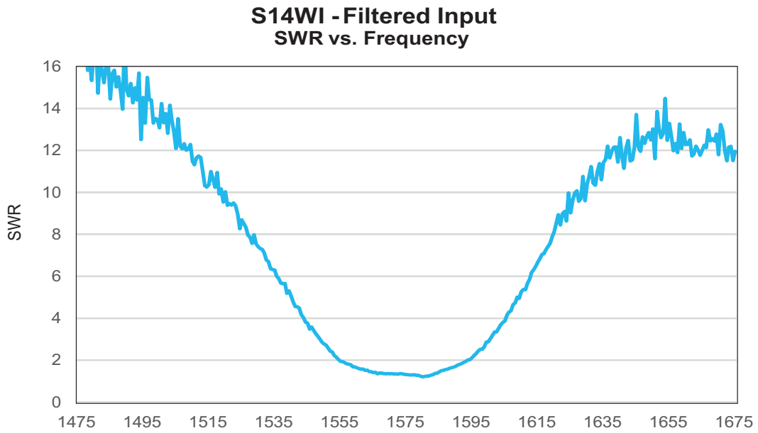
Figure 2-7. Filtered Input SWR
