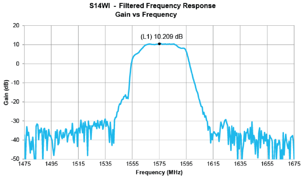
Figure 2-6. Filtered Frequency Response
