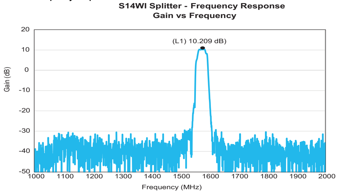
Figure 2-5. Filtered Frequency Response
