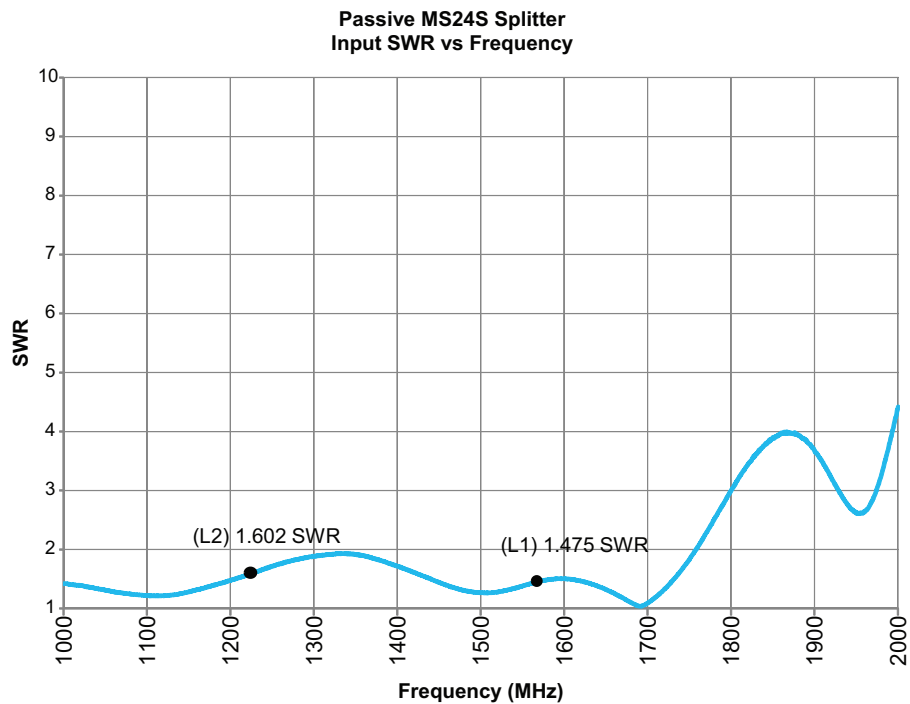
Figure 2-2. Passive MS24S Splitter Input SWR vs. Frequency
