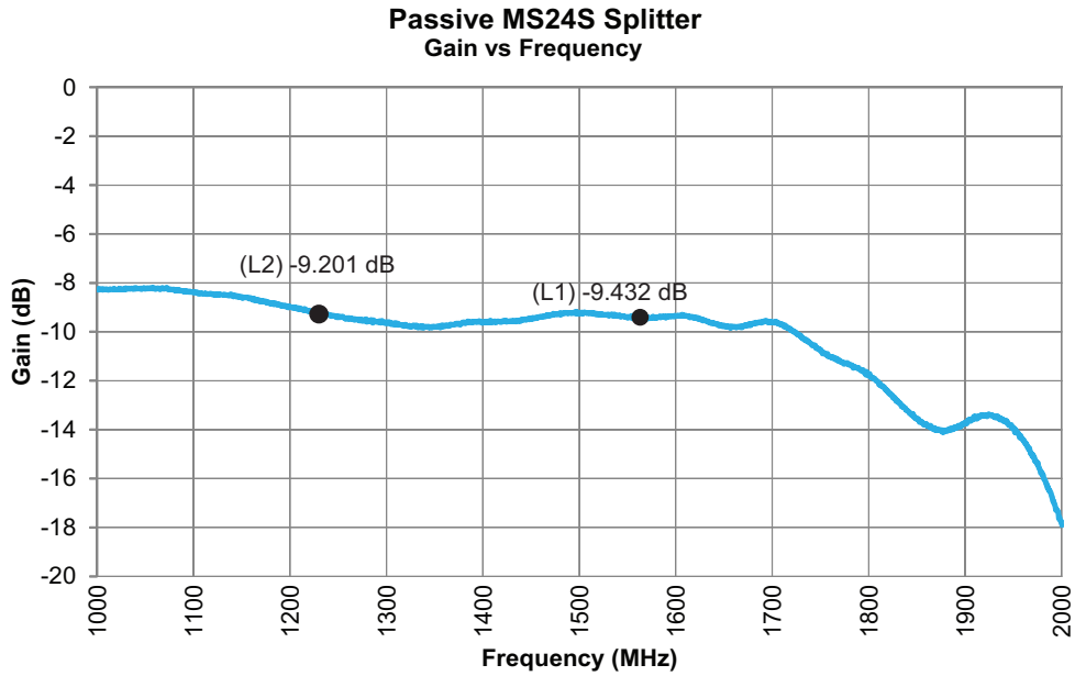
Figure 2-1. Passive MS24S Splitter Gain vs. Frequency
